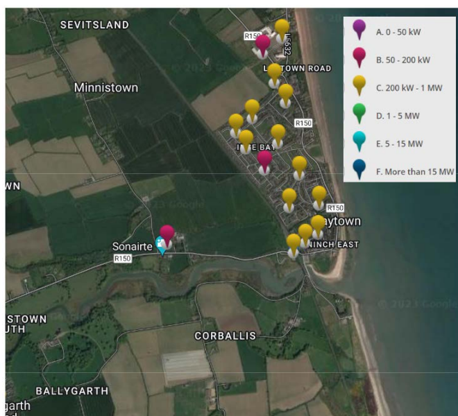
Figure 21. ESBN Generation Capacity Map
